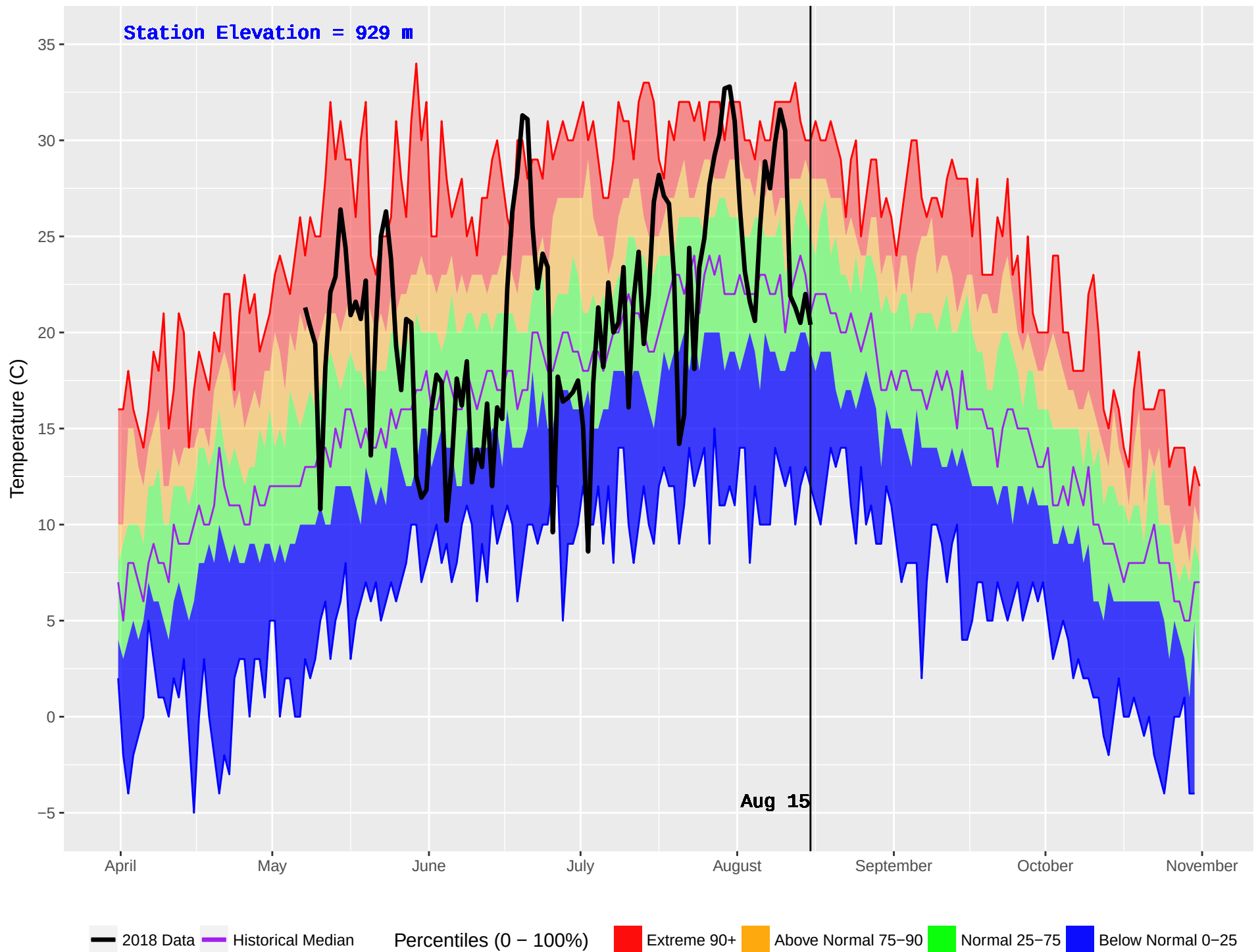
RISKE CREEK (210) : Historical (1980–2016) and Current (2018) Daily Temperature
