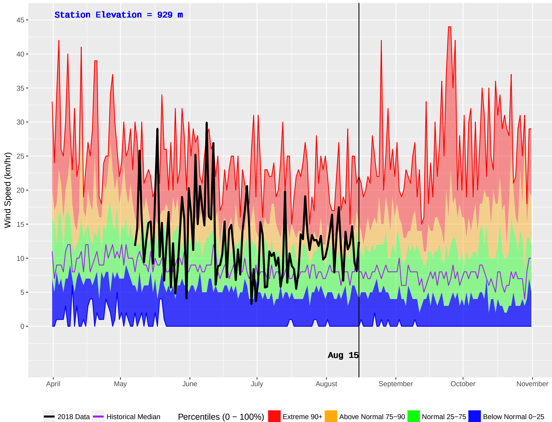
RISKE CREEK (210) : Historical (1980–2016) and Current (2018) Daily Wind Speed
