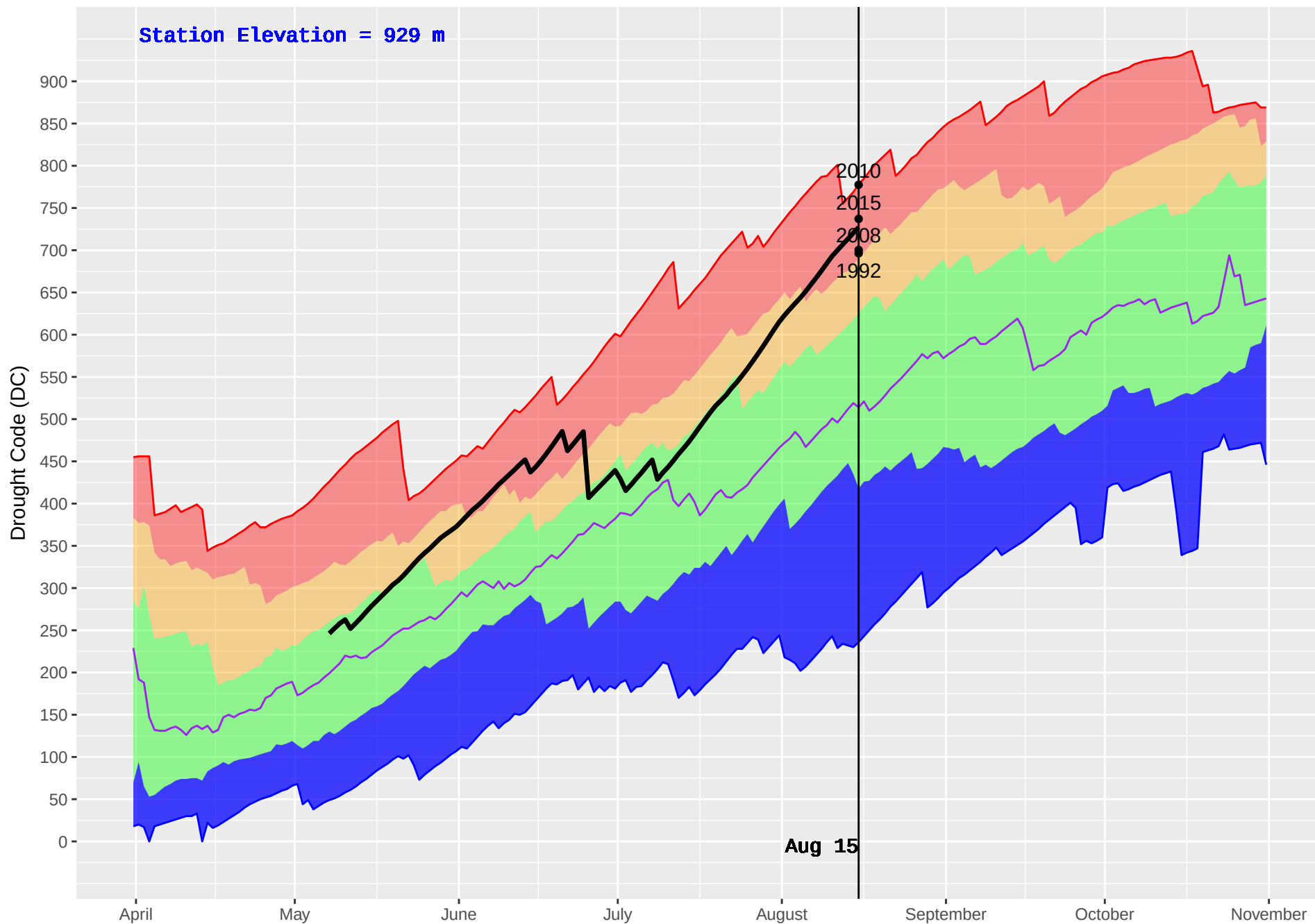
RISKE CREEK (210) : Historical (1980–2016) and Current (2018) Daily Drought Code (DC)
