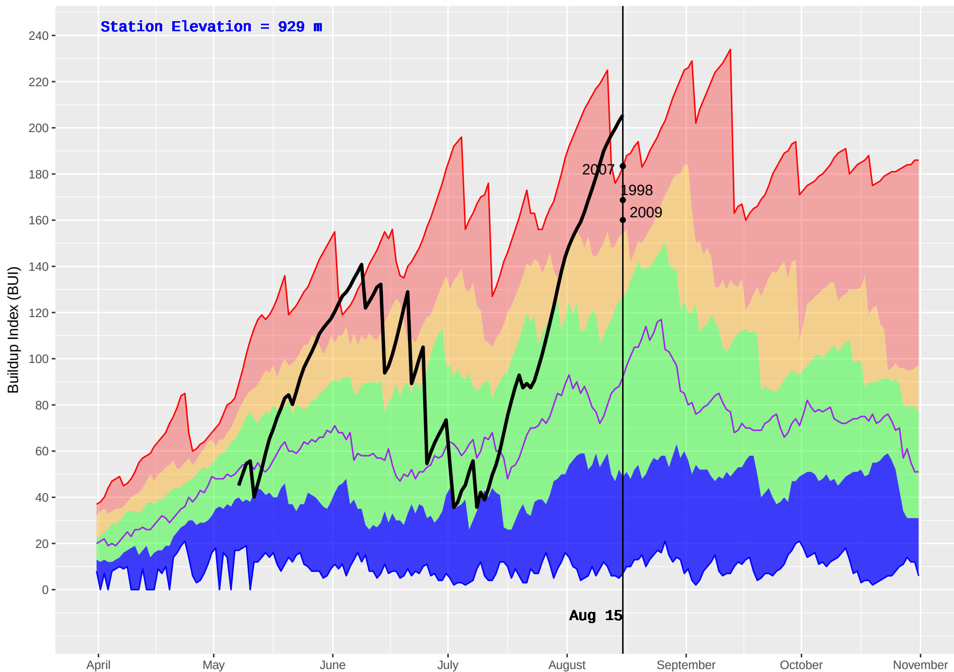
RISKE CREEK (210) : Historical (1980–2016) and Current (2018) Daily Buildup Index (BUI)
