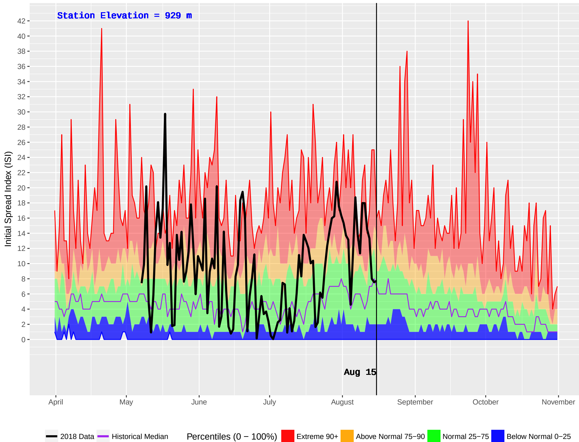
RISKE CREEK (210) : Historical (1980–2016) and Current (2018) Daily Initial Spread Index (ISI)
