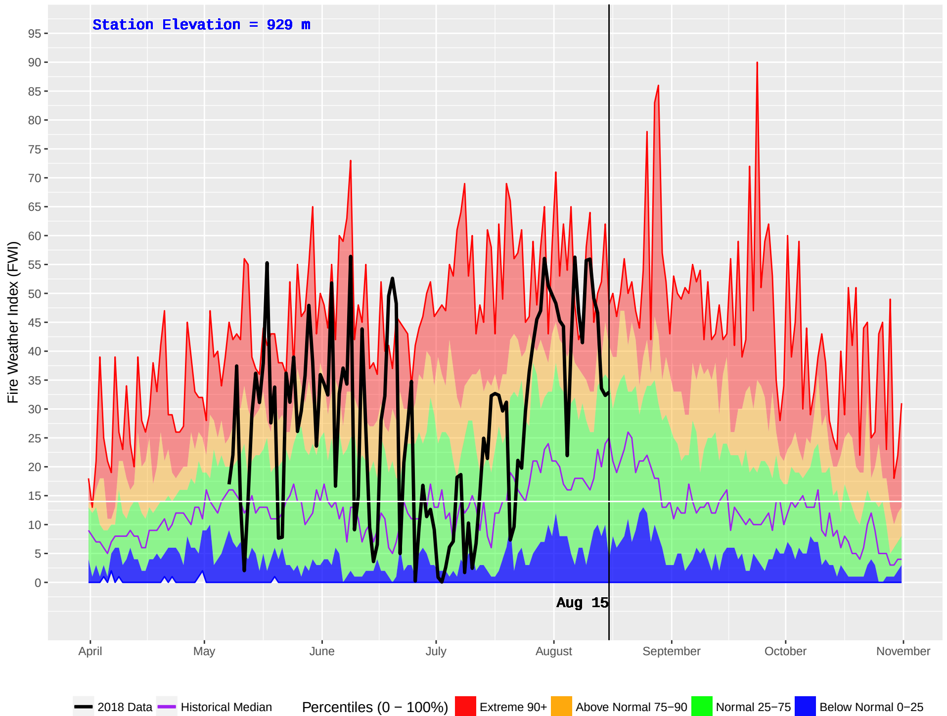
RISKE CREEK (210) : Historical (1980–2016) and Current (2018) Daily Fire Weather Index (FWI)
