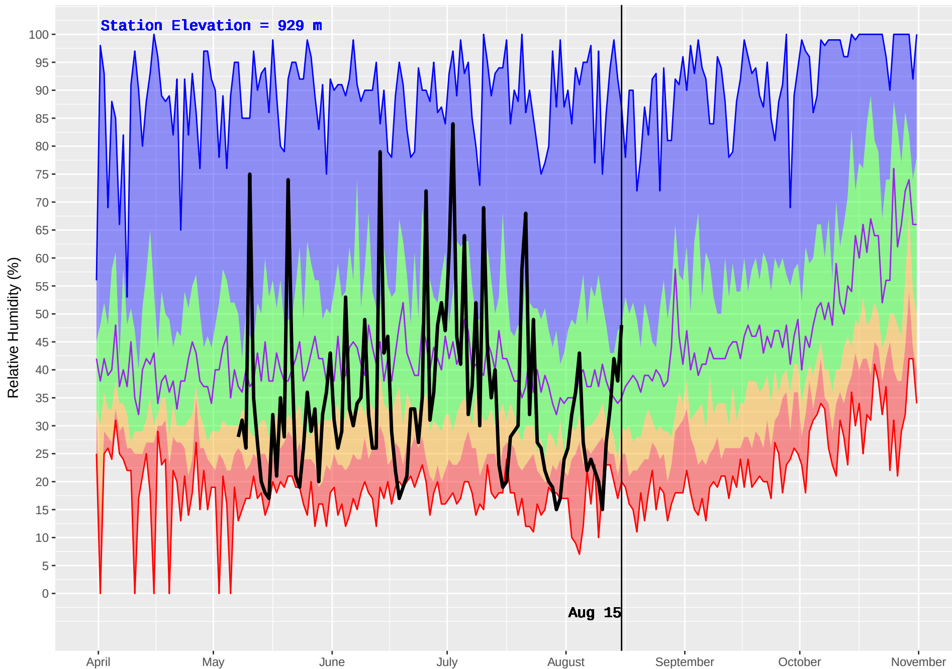
RISKE CREEK (210) : Historical (1980–2016) and Current (2018) Daily Relative Humidity
